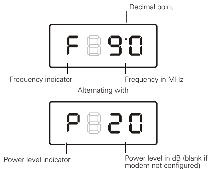
Figure 4-8 RF upstream modem front panel display
