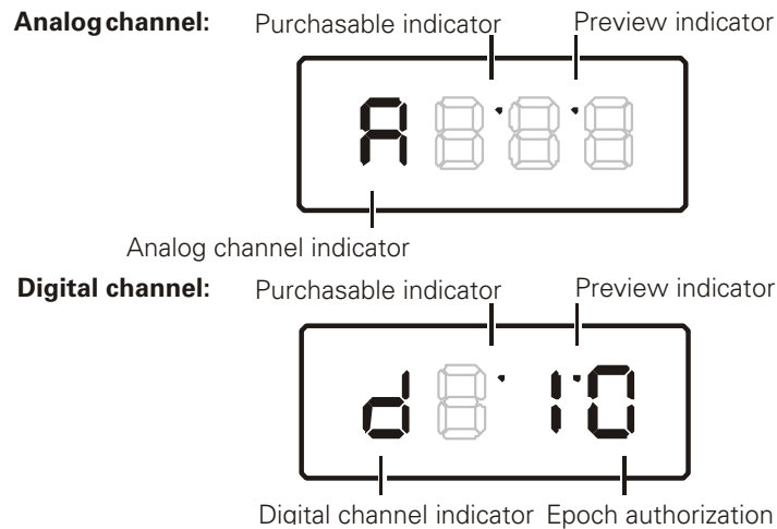
Figure 4-7 Current channel status front panel displays
